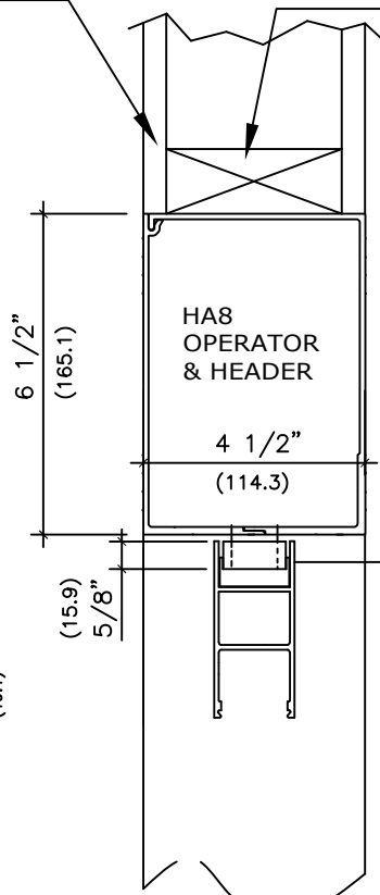
VERTICAL SECTION
