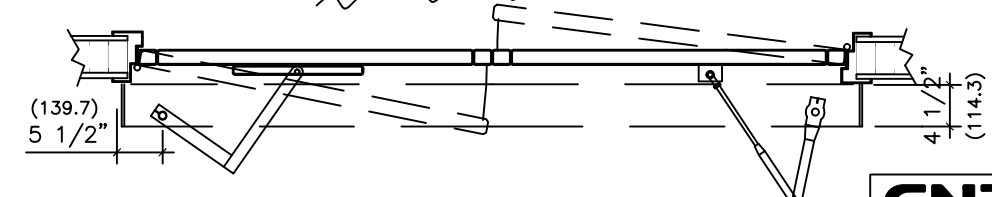
3 HORIZONTAL SECTION
