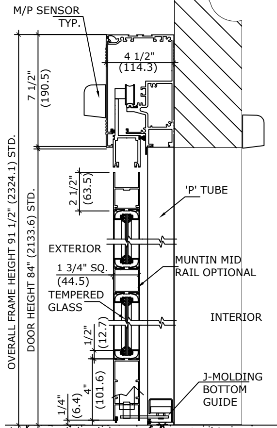
2 VERTICAL SECTION
