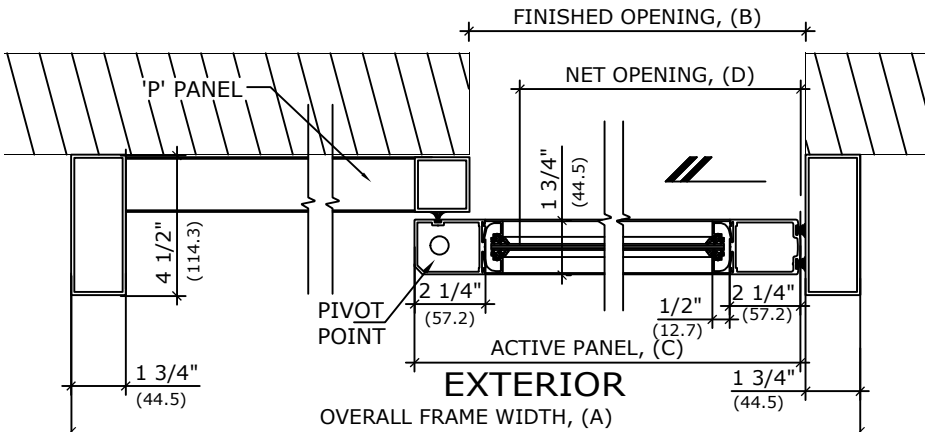
1 HORIZONTAL SECTION
