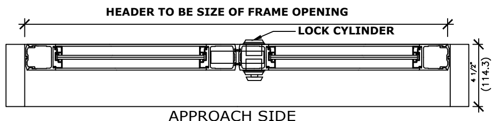
HORIZONTAL SECTION
