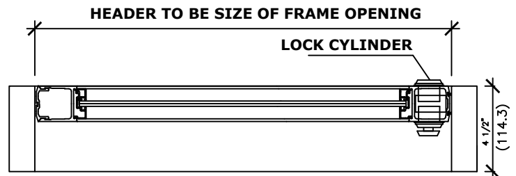
HORIZONTAL SECTION
