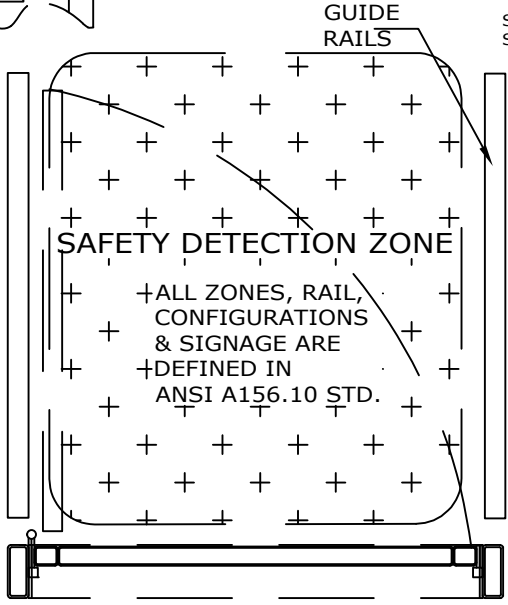
ELEVATION OF DOOR
