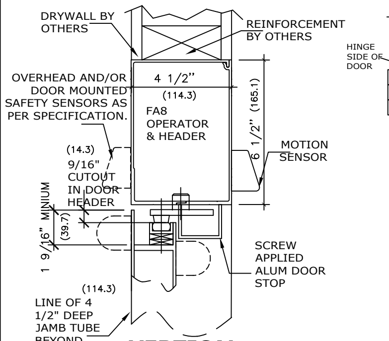
VERTICAL SECTION
