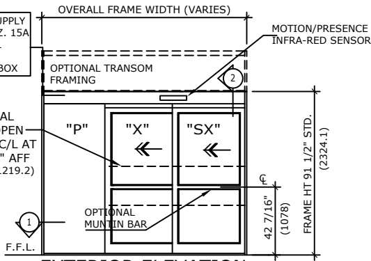
EXTERIOR ELEVATION
