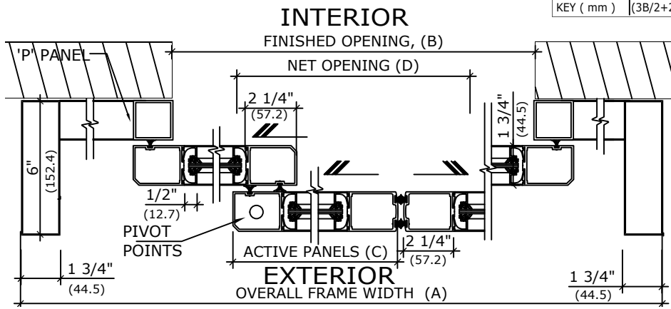
1 HORIZONTAL SECTION
