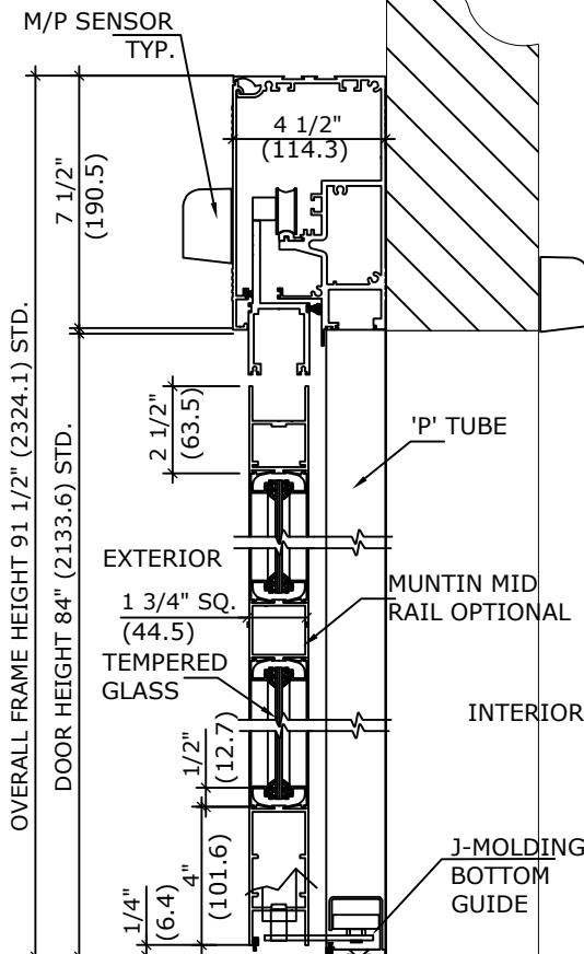
2 VERTICAL SECTION
