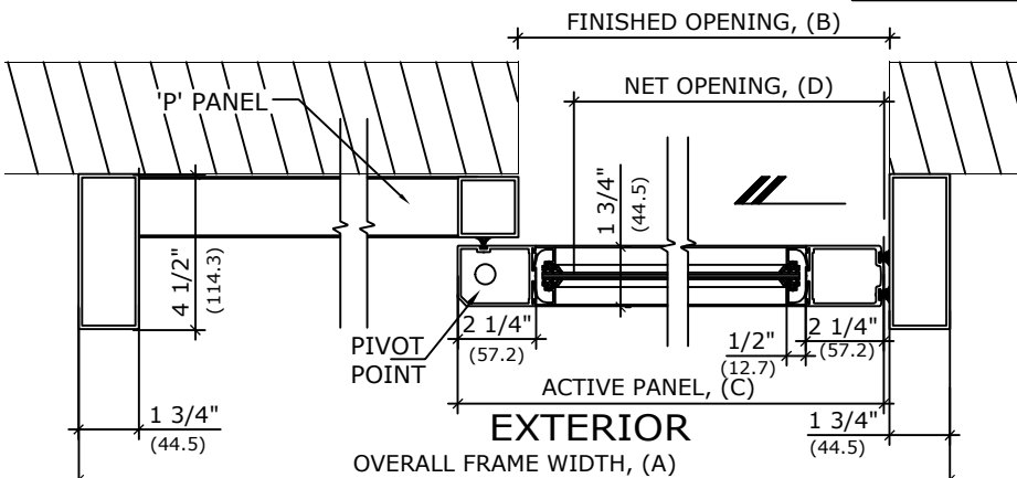
1 HORIZONTAL SECTION
