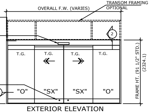
EXTERIOR ELEVATION
